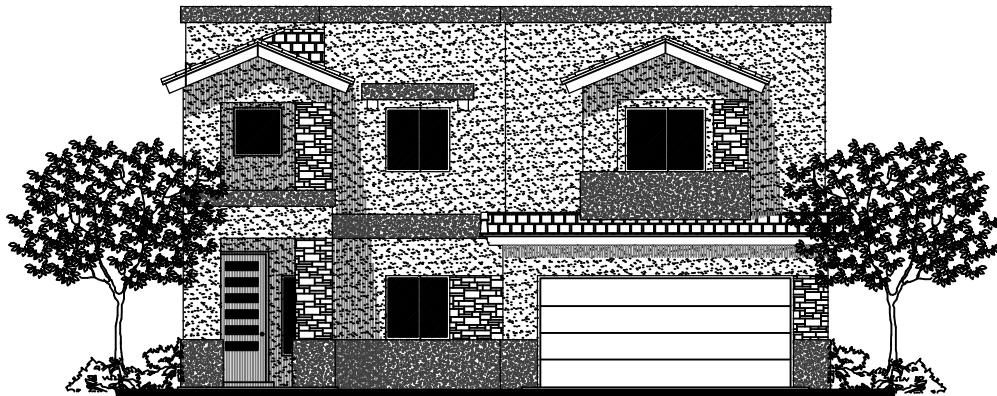
Y - ELEVATION (FLAT ROOF)
