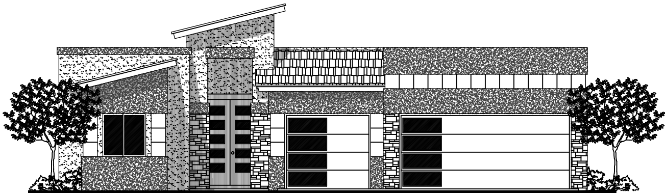
Y - ELEVATION (FLAT ROOF)
